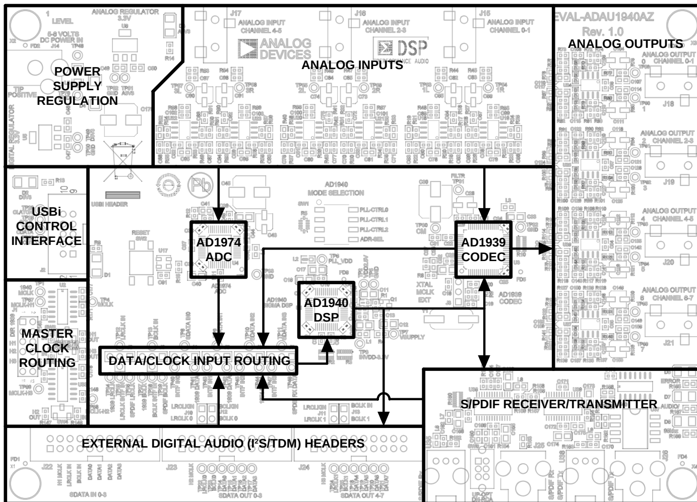
Figure 2. Board Layout Block Diagram
