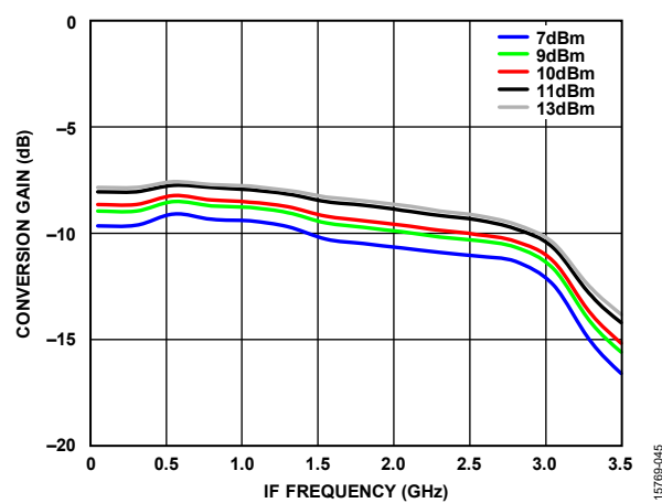
Figure 45. Conversion Gain vs. IF Frequency at Various LO Drives
