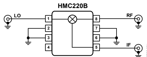
Figure 51. Typical Applications Circuit
