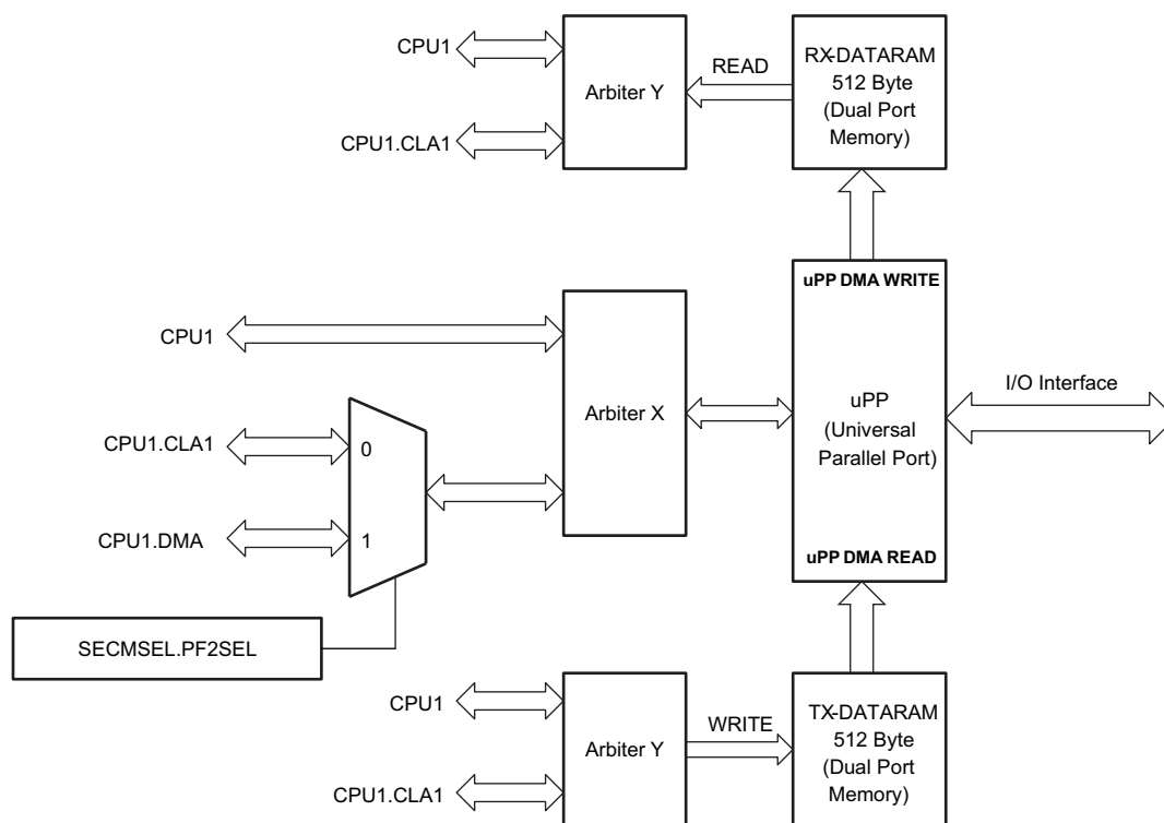
Figure 4-78. uPP Integration
