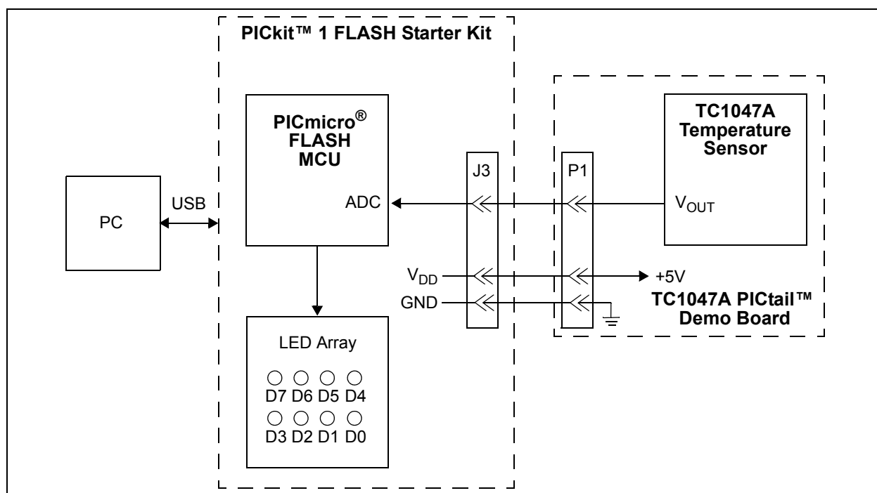
FIGURE 2-1: TC1047A Temperature-to-Voltage Converter PICtail™ Demo Board Block Diagram.
