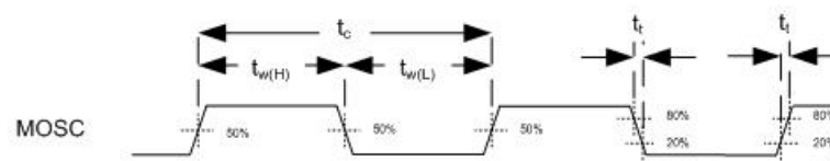
Figure 1. System Oscillators
