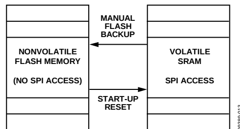
Figure 12. SRAM and Flash Memory Diagram
