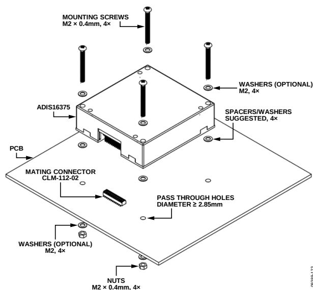
Figure 23. Mounting Example
