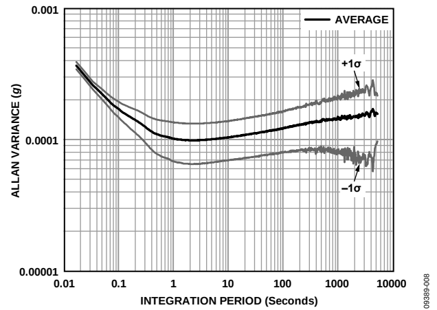
Figure 8. Accelerometer Allan Variance, 25°C
