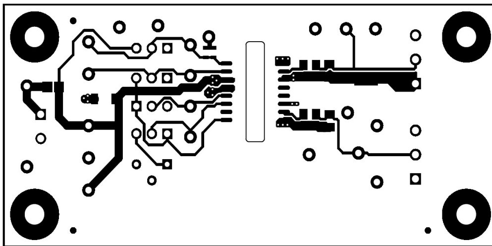
Figure 9. Top Layer
