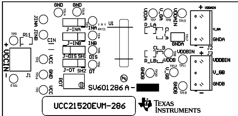
Figure 8. Top Overlay
