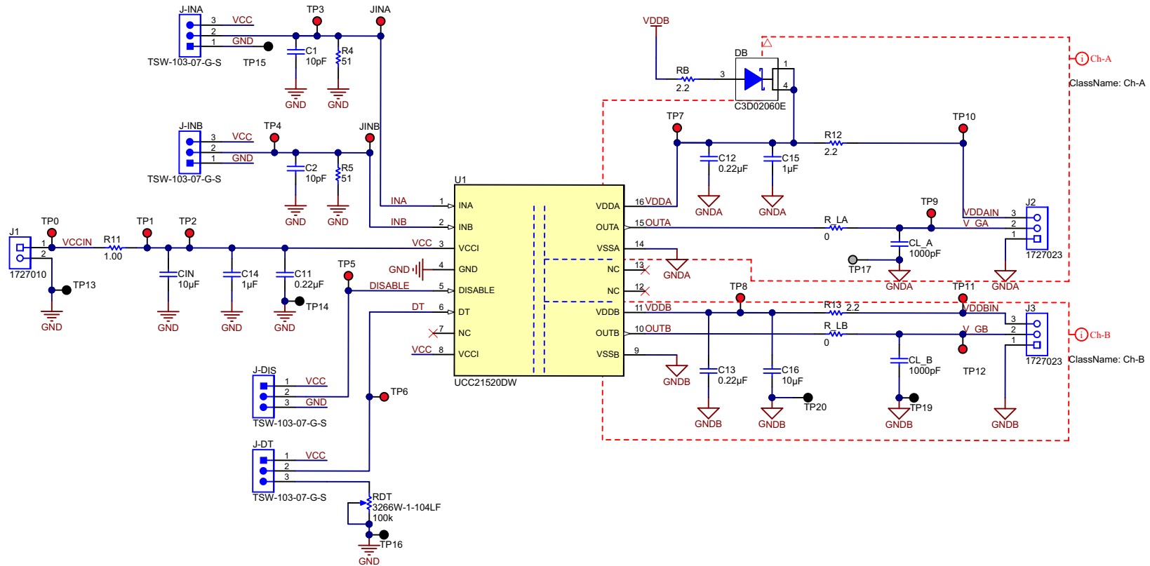
Figure 7. UCC21520EVM-286 Schematic
