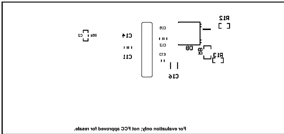
Figure 11. Bottom Overlay
