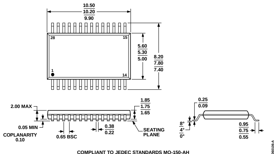
Figure 25. 28-Lead Shrink Small Outline Package [SSOP]
