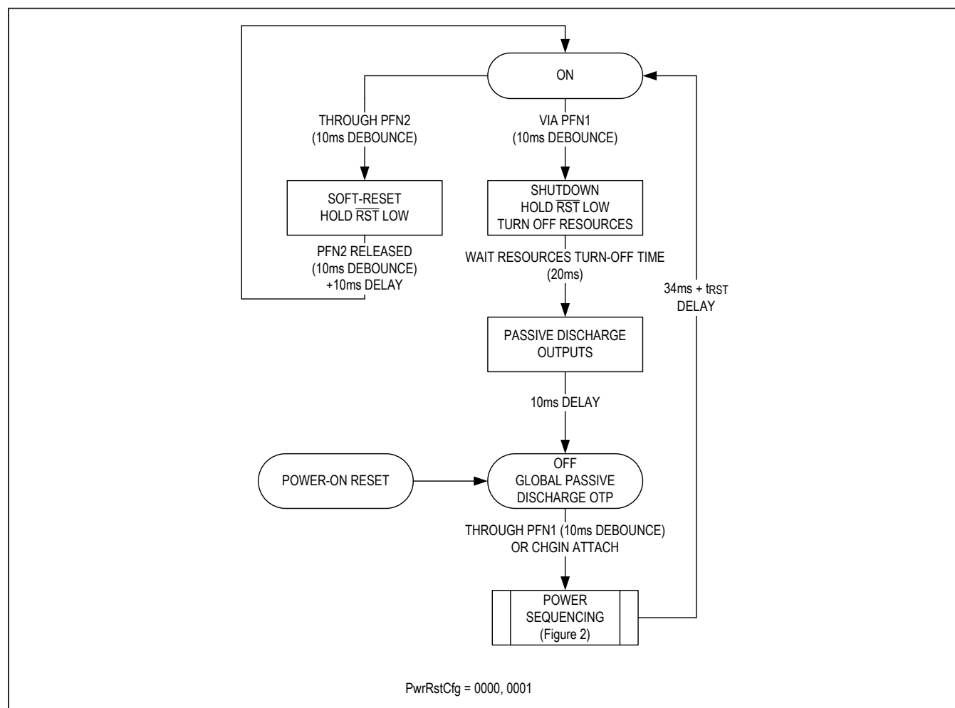
Figure 1a. PwrRstCfg = 0000,0001
