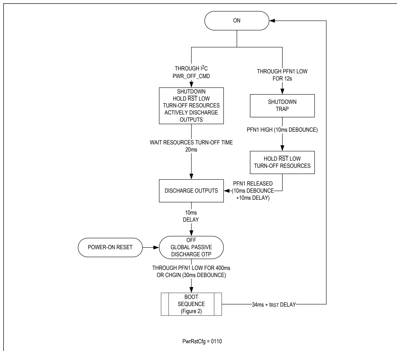
Figure 1d. PwrRstCfg = 0110
