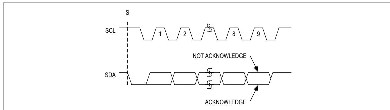
Figure 20. Acknowledge Bits
