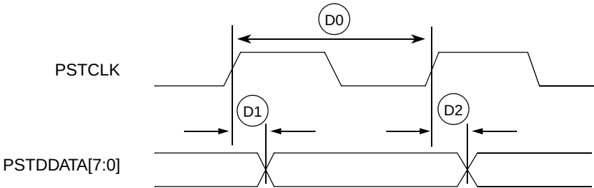
Figure 27. Real-Time Trace AC Timing
