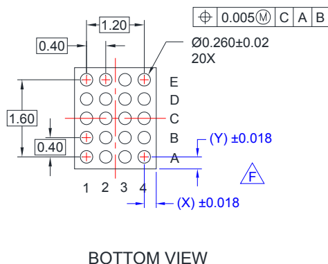
Figure 34. 2 x 1.82 mm, 20-Bump, 0.4 mm Pitch, Wafer-Level Chip-Scale Package (WLCSP)
