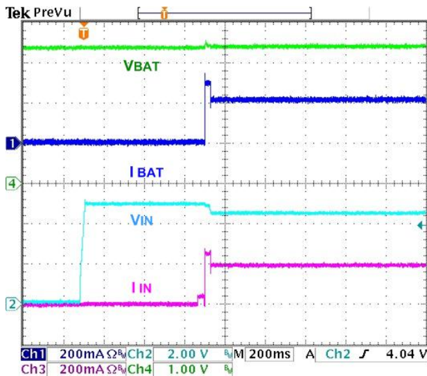
Figure 14. Auto-Charge Startup with 200 mA Limited Charger / Adaptor, V_{BAT} = 3.4\text{ V}
