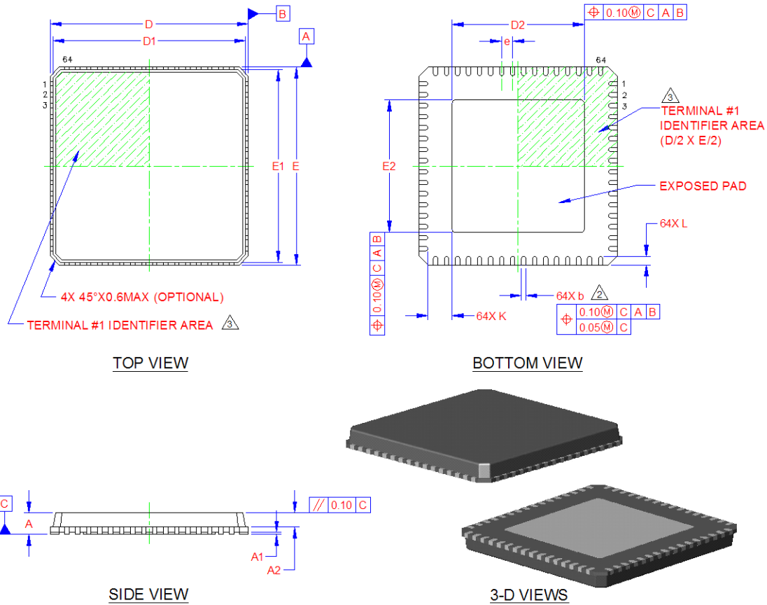
Figure 2 USB5434B 64 Pin QFN Package
