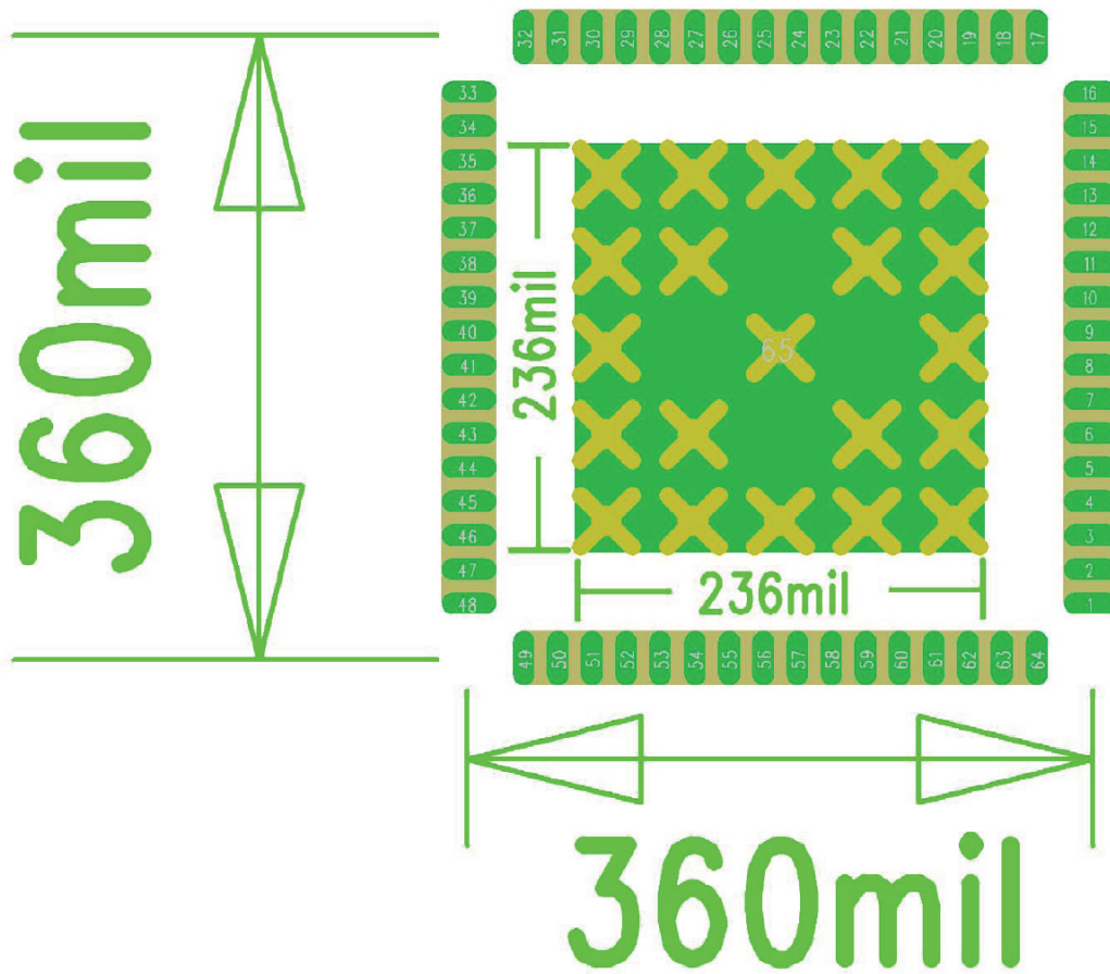
Figure 3 Recommended PCB Land Pattern
