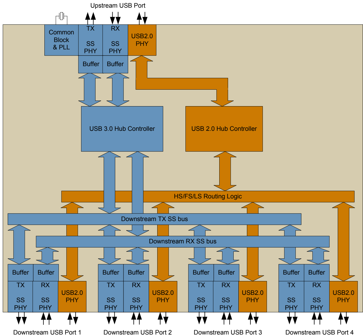
Figure 1 USB5434B Block Diagram
