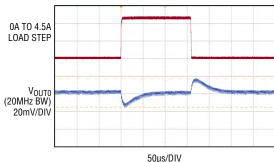
Figure 7. Output Voltage V_{OUT0} vs Load Current ( V_{OUT0} = 1.0V ), Measured by 1X Probe on C_{OUT8}
