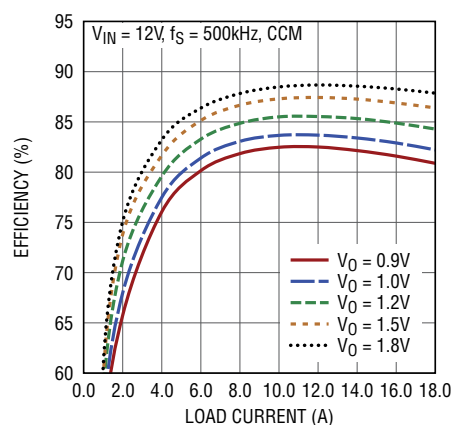
Figure 6. Efficiency vs Load Current at V_{IN} = 12V
