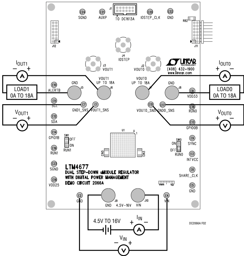
Figure 2. Proper Measurement Equipment Setup
