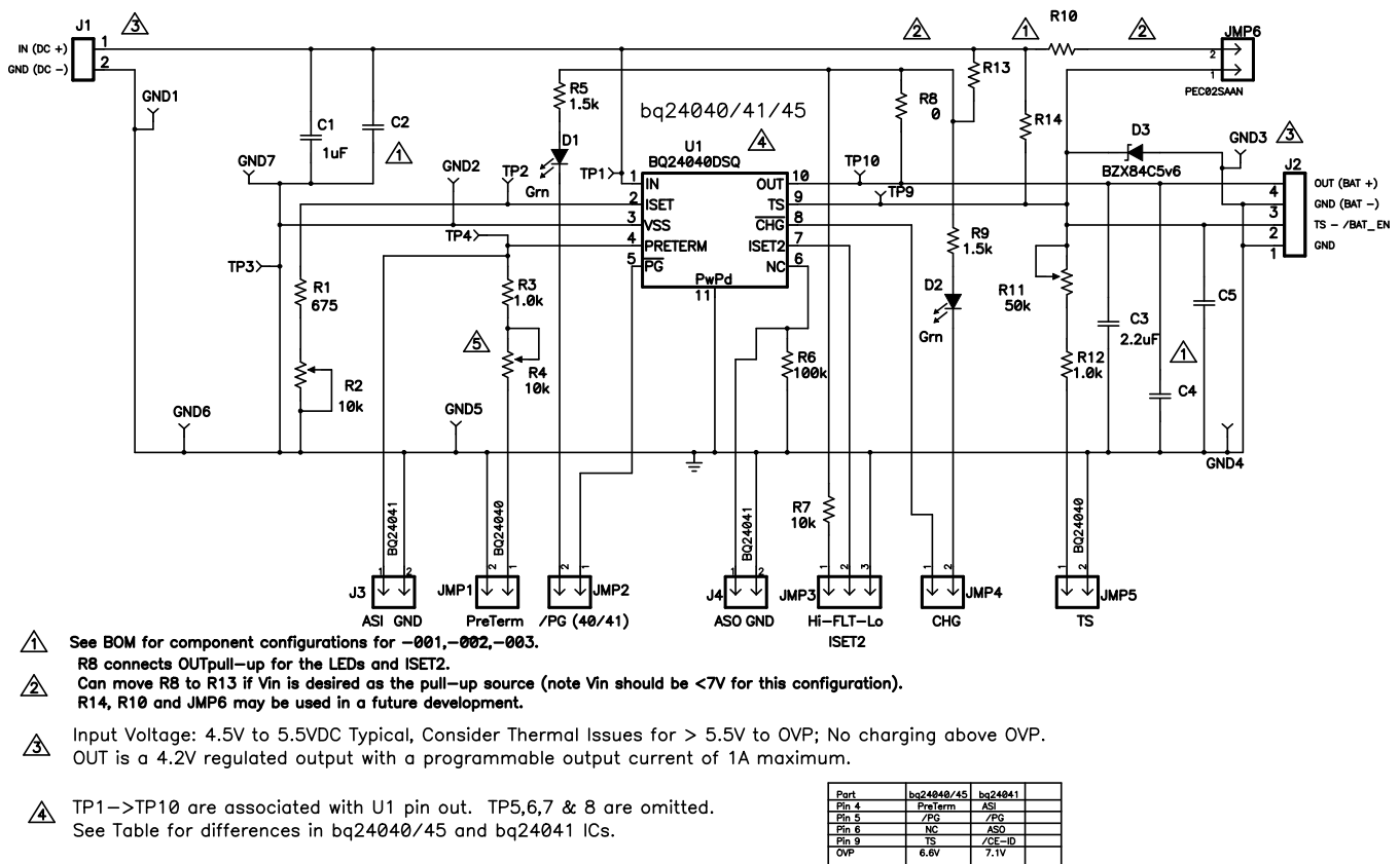
Figure 3. bq2404x EVM Board Schematic
