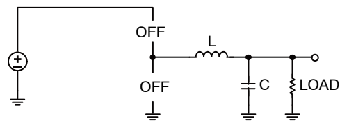
Figure 25. Buck Topology Inductor Current During t_2 and t_3
