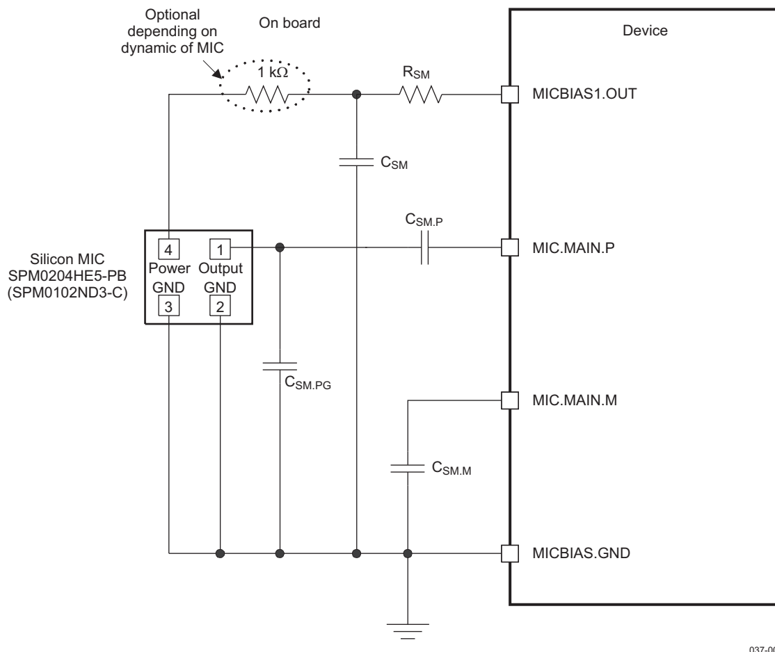
Figure 6-8. Silicon Microphone
