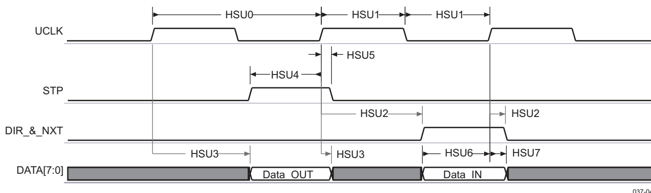
Figure 5-14. HS-USB Interface—Transmit and Receive Modes (ULPI 8-bit)
