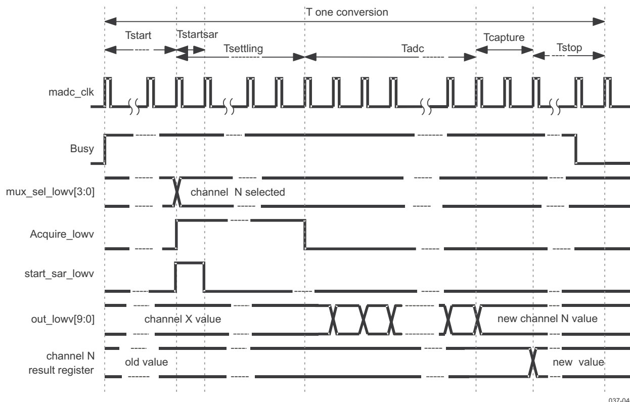
Figure 5-17. Conversion Sequence General Timing Diagram
