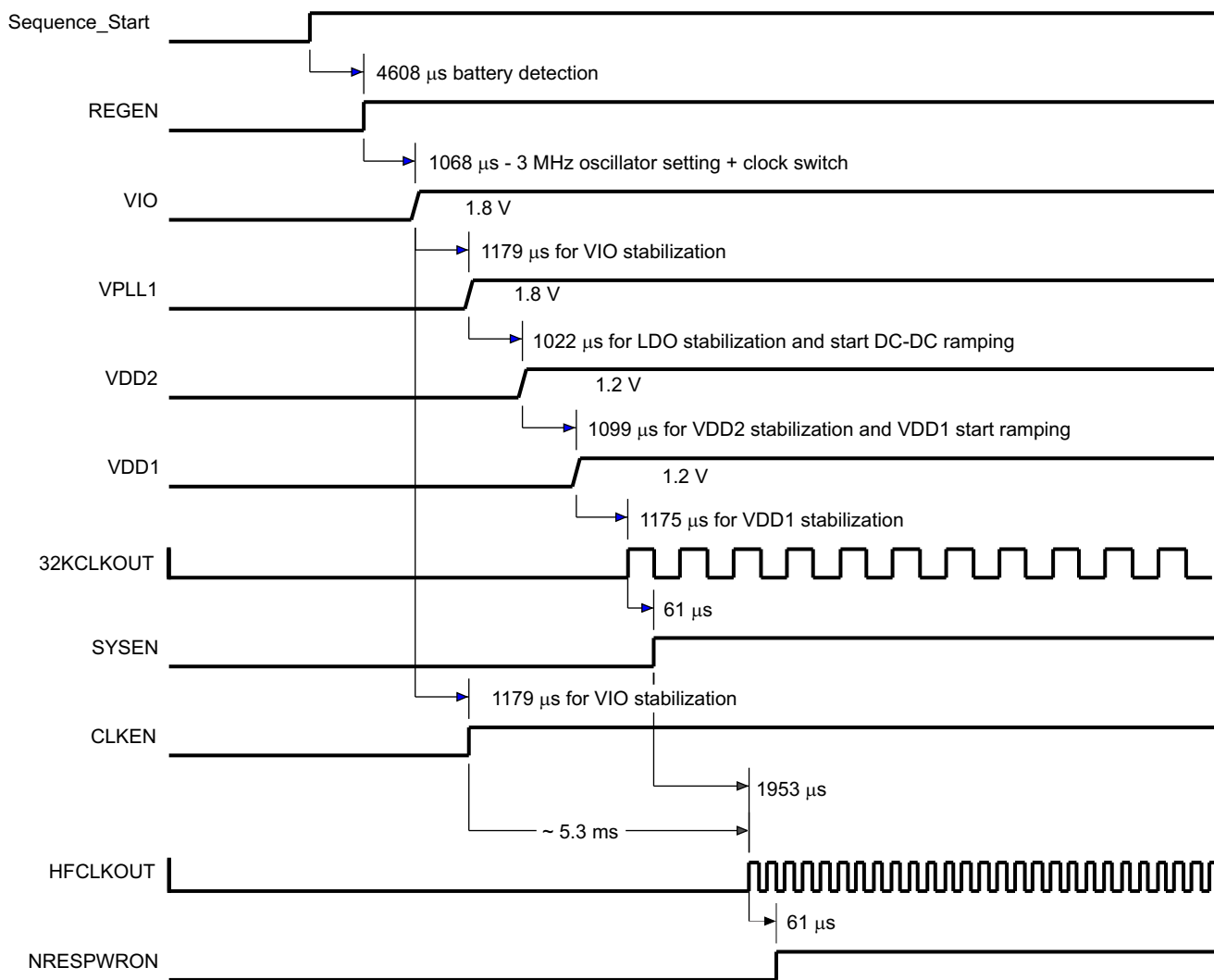
Figure 5-9. Timings–Power On in OMAP3 Mode
