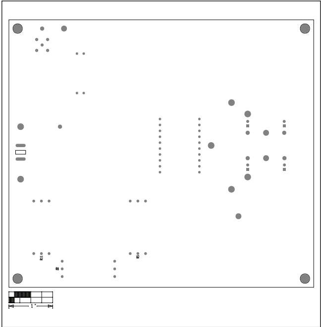
Bottom Silkscreen
