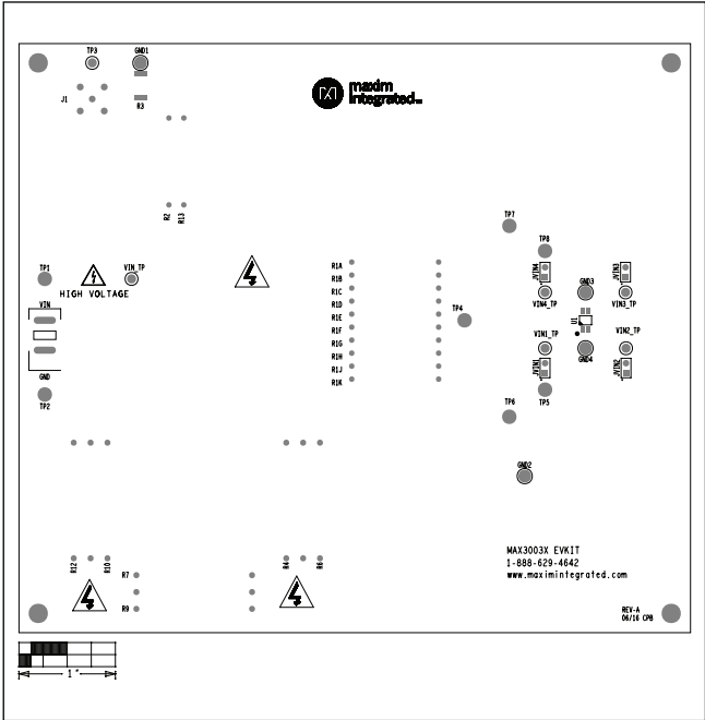
Top Silkscreen
