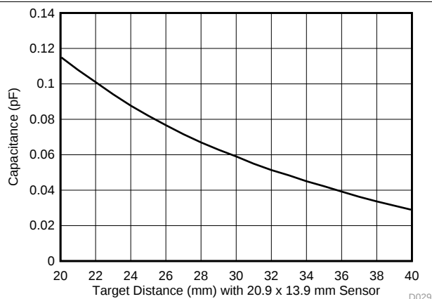
Figure 58. FDC2212 / FDC2214: Capacitance vs Target Distance (20 to 40 mm)
