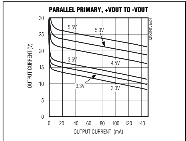
Figure 4. T1 Parallel Primary: \pm VOUT Voltage vs. Output Current (+VOUT to -VOUT Loading)
