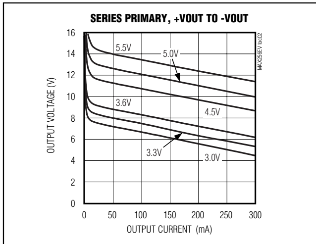
Figure 2. T1 Series Primary: \pm VOUT Voltage vs. Output Current (+VOUT to -VOUT Loading)
