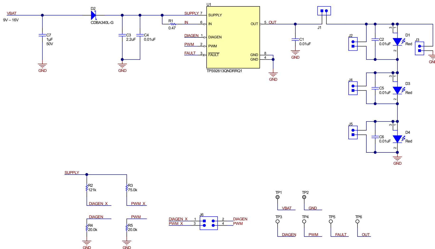
Figure 4. TPS92613EVM Schematic
