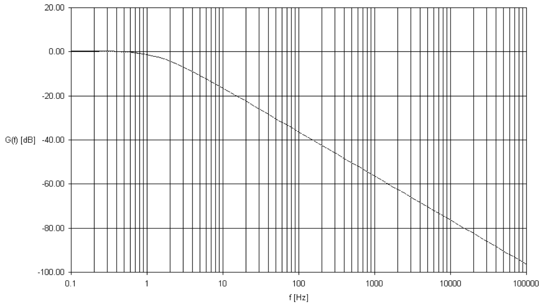
Figure 10 - DPLL Jitter Transfer Function Diagram - wide range of frequencies
