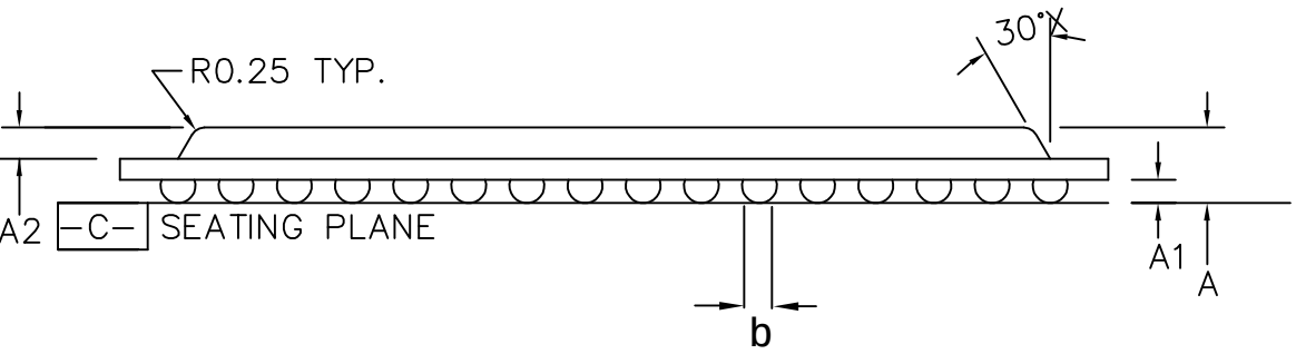
SIDE VIEW
