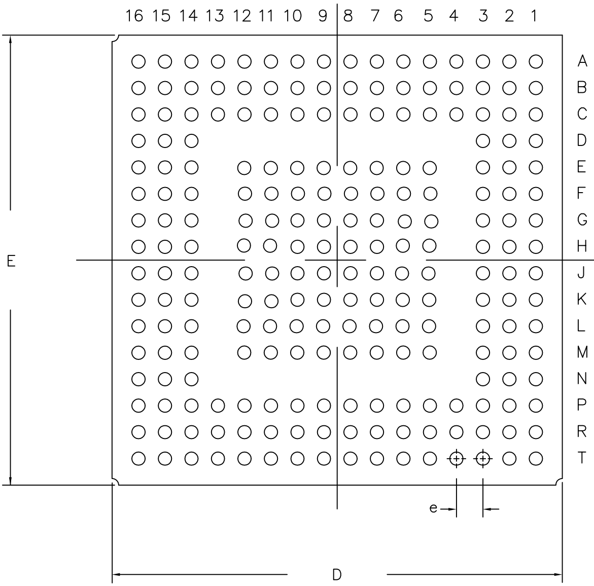
BOTTOM VIEW
