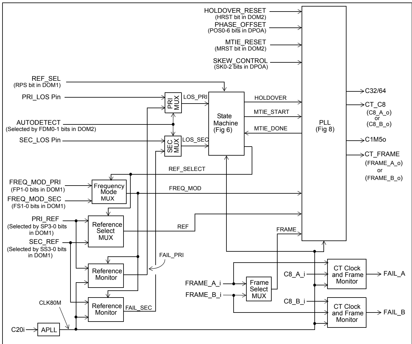
Figure 6 - DPLL Functional Block Diagram
