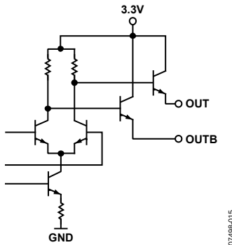
Figure 19. LVPECL Output Simplified Equivalent Circuit
