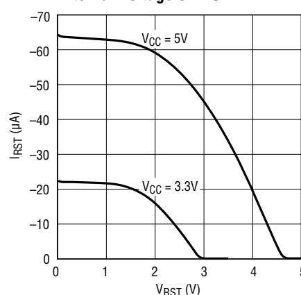
RST Pull-Up Current vs External Voltage on RST
