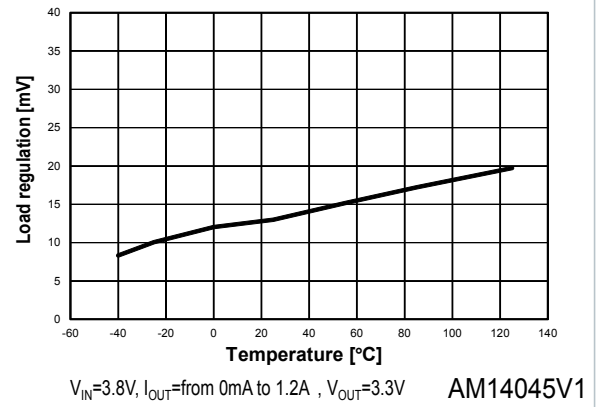
Figure 13. Load regulation vs. temperature
