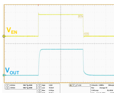
Figure 29. Turn-on time
