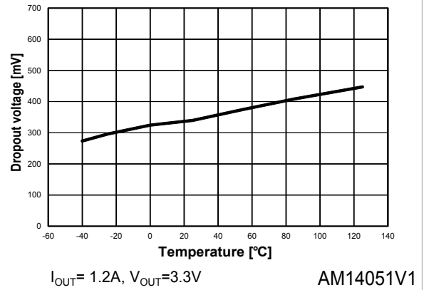
Figure 19. Dropout voltage vs. temperature (I_{OUT} = 1.2 \text{ A})
