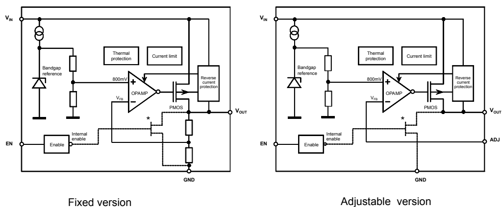
Figure 2. Block diagram
