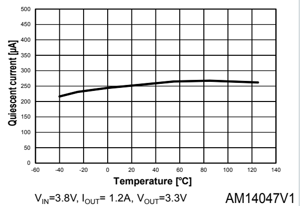
Figure 15. Quiescent current vs. temperature ( I_{OUT} = 1.2 A)
