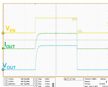
Figure 28. Enable transient
