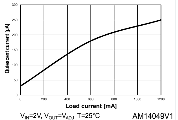
Figure 17. Quiescent current vs. load current
