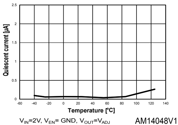
Figure 16. Shutdown current vs. temperature
