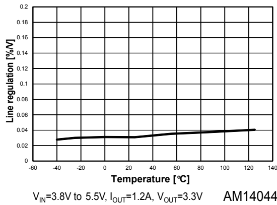
Figure 12. Line regulation vs. temperature
