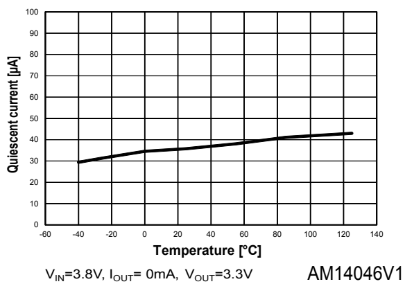
Figure 14. Quiescent current vs. temperature ( I_{OUT} = 0 mA)
