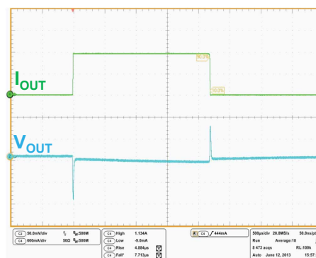
Figure 27. Load transient
