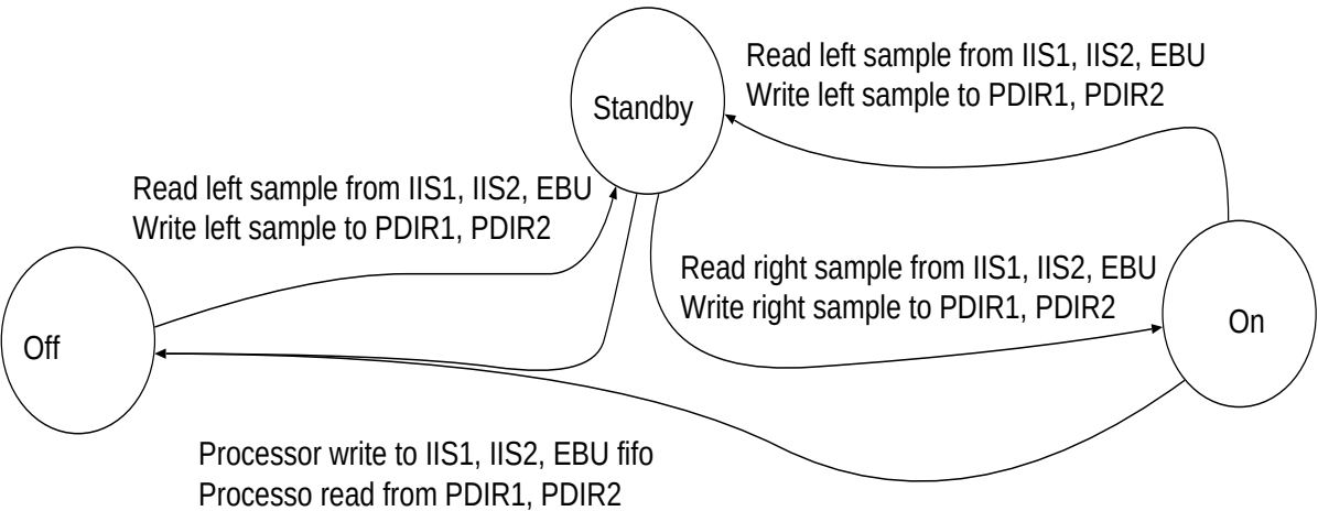
Figure 17-7 Automatic Resynchronization FSM of left-right FIFOs
