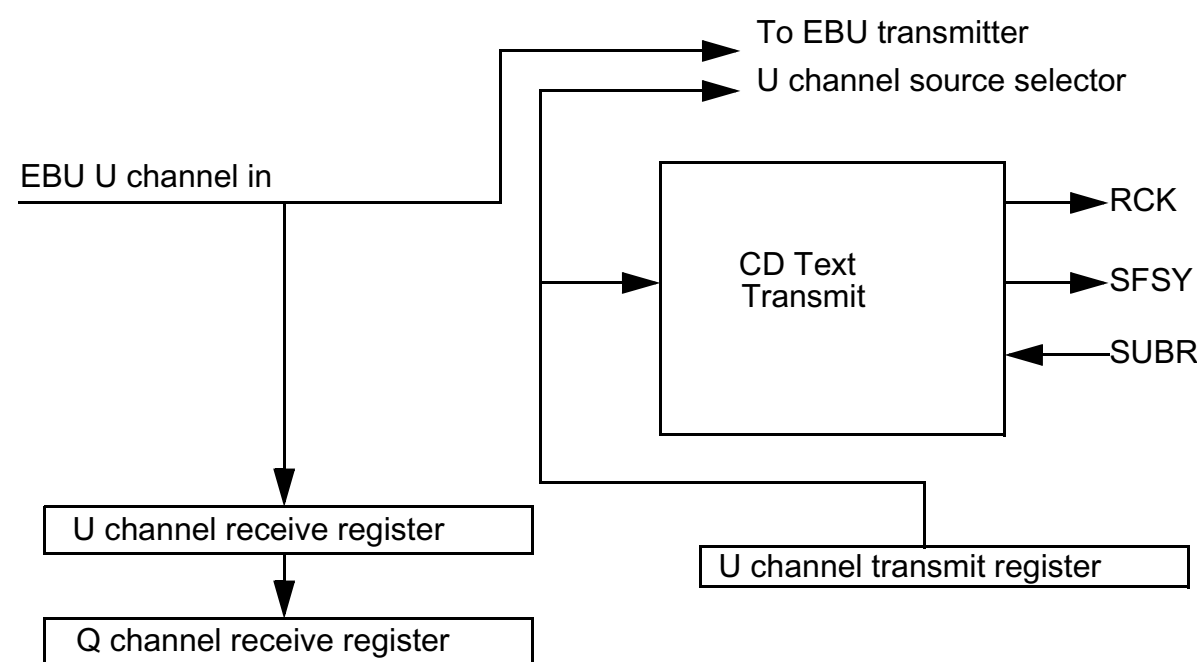
Figure 17-4 CD-Subcode Interface
