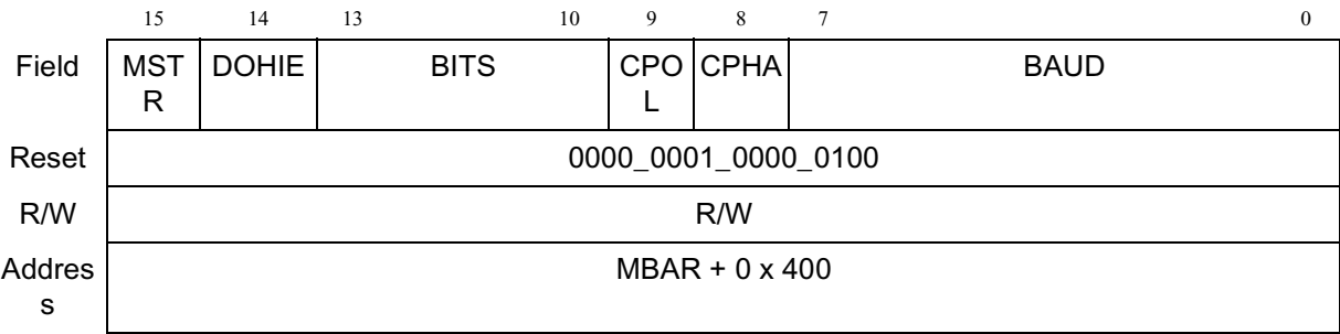
Figure 16-3 QSPI Mode Register (QSPIMR)
