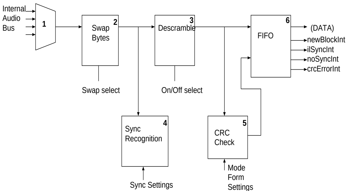
Figure 17-9 Block Decoder
