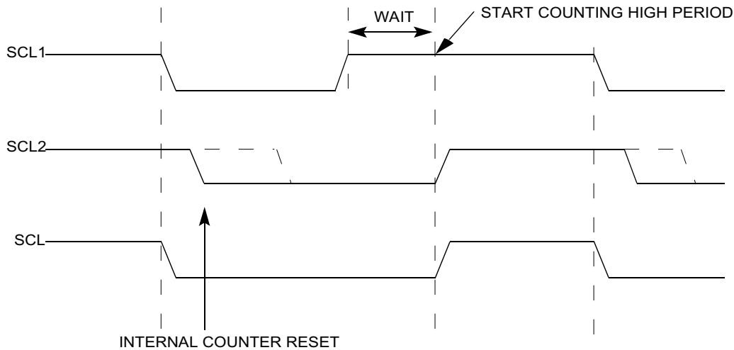
Figure 18-3 Synchronized Clock SCL
