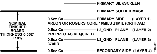
Figure 27. 4-Layer Stackup
