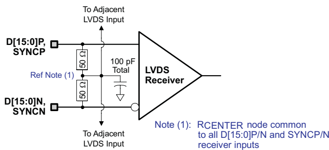
Figure 33. D[15:0]P/N and SYNCN LVDS Input Configuration
