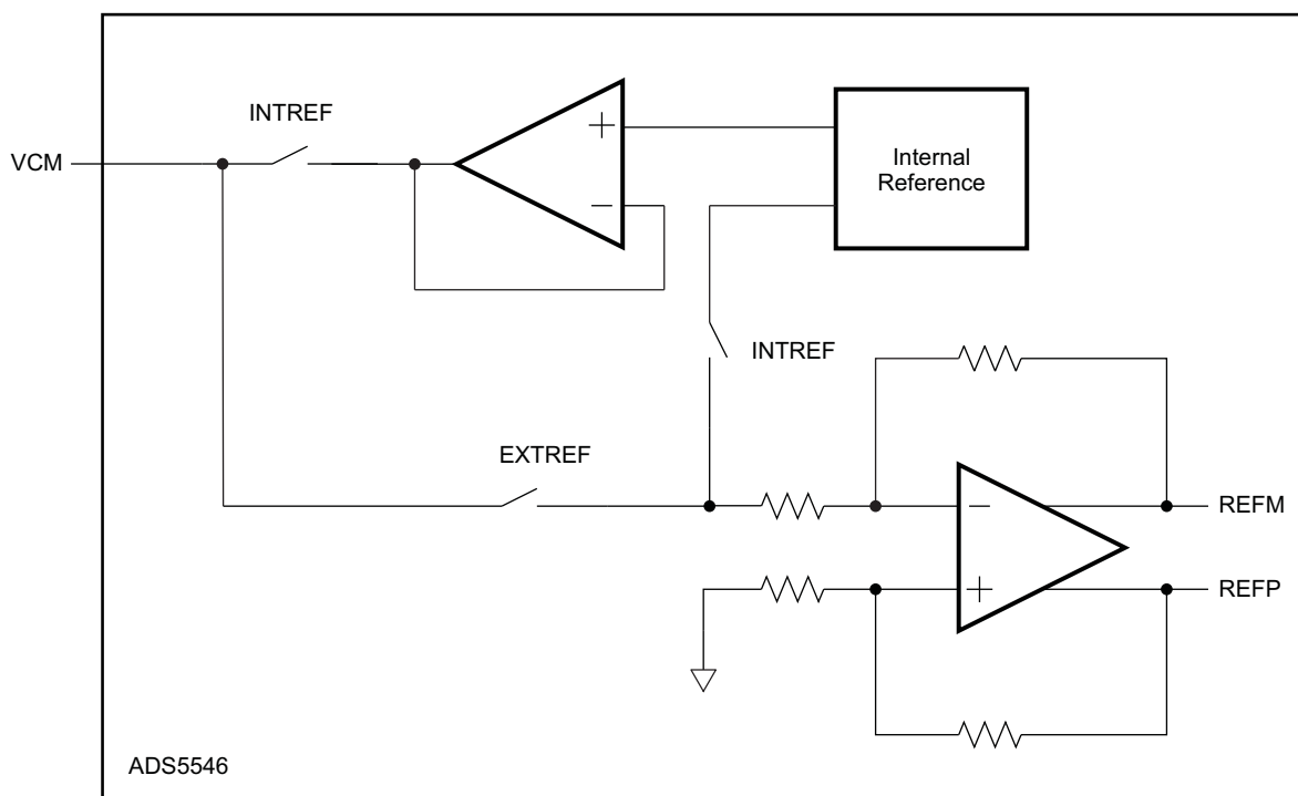
Figure 49. Reference Section
