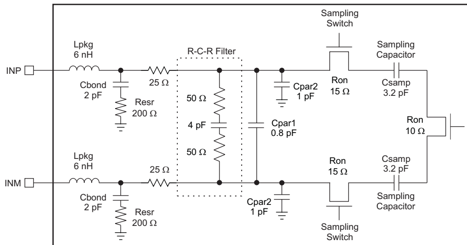
Figure 41. Input Stage
