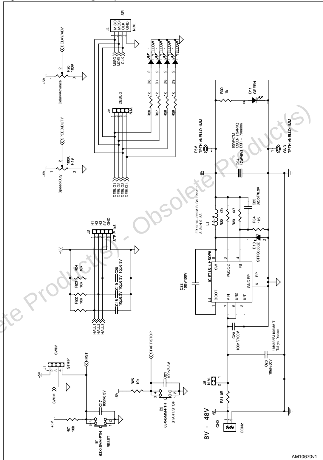
Figure 2. Schematic (part 2)
