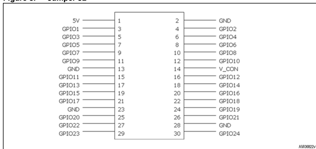
Figure 8. Jumper J2
