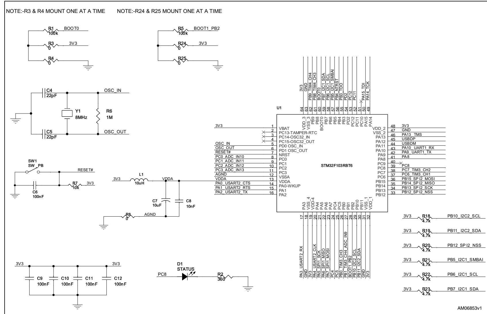
Figure 30. Microcontroller section
