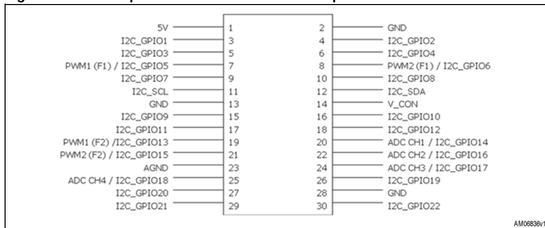
Figure 17. J2 Interpretation for I 2 C interface of 30-pin header
