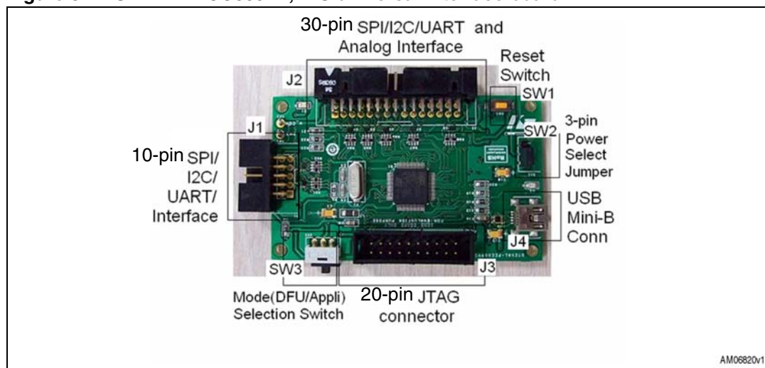
Figure 6. STEVAL-PCC009V2, IBU universal interface board
