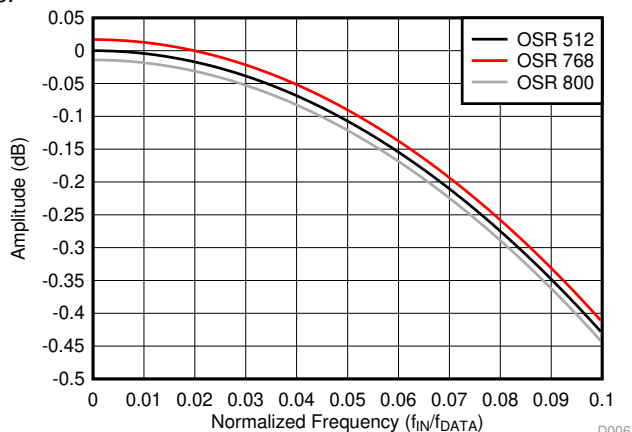
Figure 50. Non-Binary OSR Sinc 3 Filter Frequency Response
