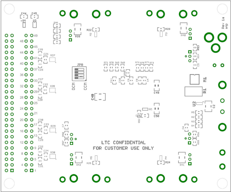
DC2363A Bottom
