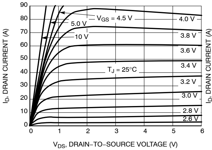
Figure 1. On-Region Characteristics
