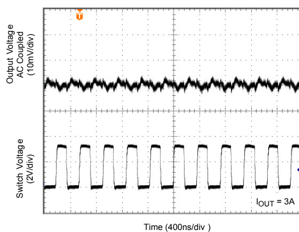
Output Ripple
