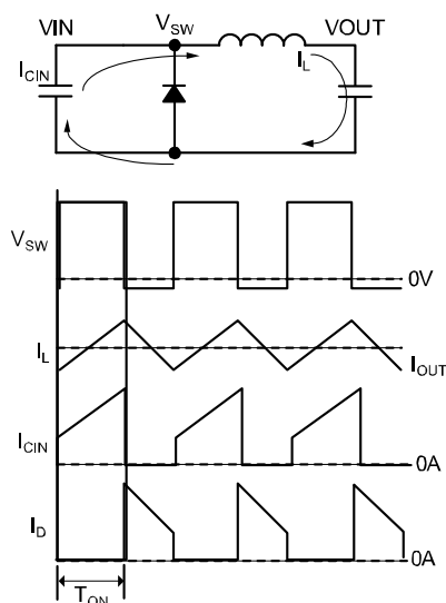
Figure 3. On-Time
