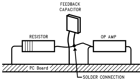
Figure 29. Air Wiring
