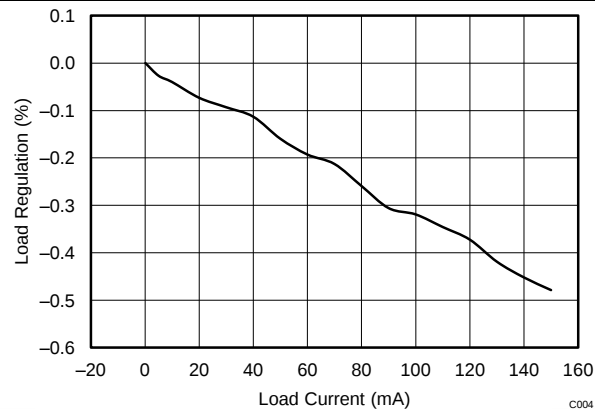
Figure 11. Load Current vs Load Regulation
