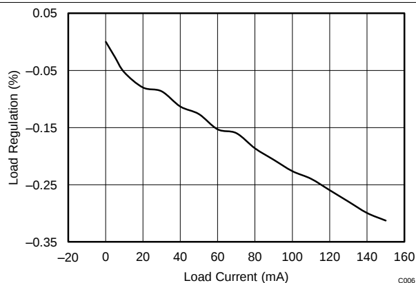
Figure 13. Load Current vs Load Regulation
