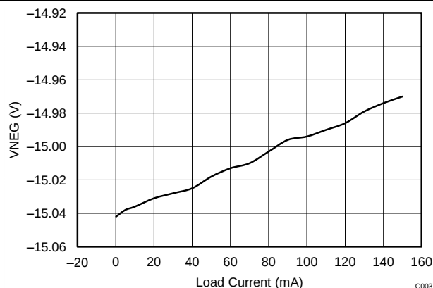
Figure 10. Load Current vs VNEG
