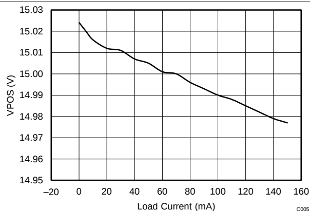
Figure 12. Load Current vs VPOS
