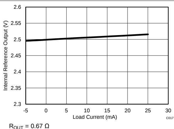
Figure 83. Internal Reference Output Impedance
