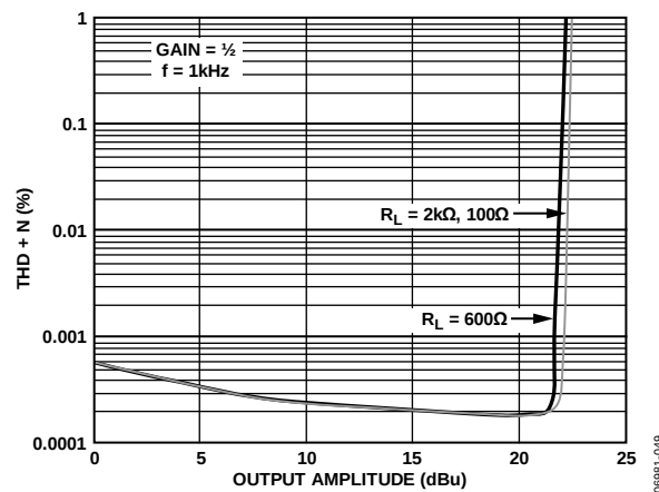
Figure 33. THD + N vs. Output Amplitude, G = \frac{1}{2}
