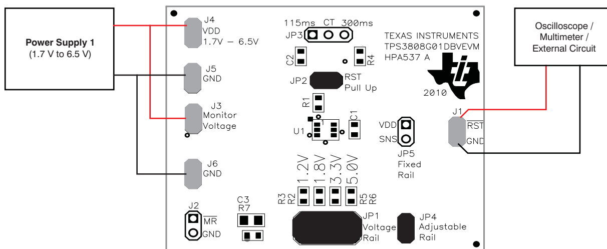
Figure 1. Using the TPS3808G01EVM as a Single-Rail Monitor
