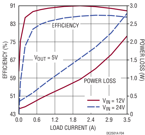
Figure 4. DC2501A Efficiency vs Load Current (T A = 25°C)
