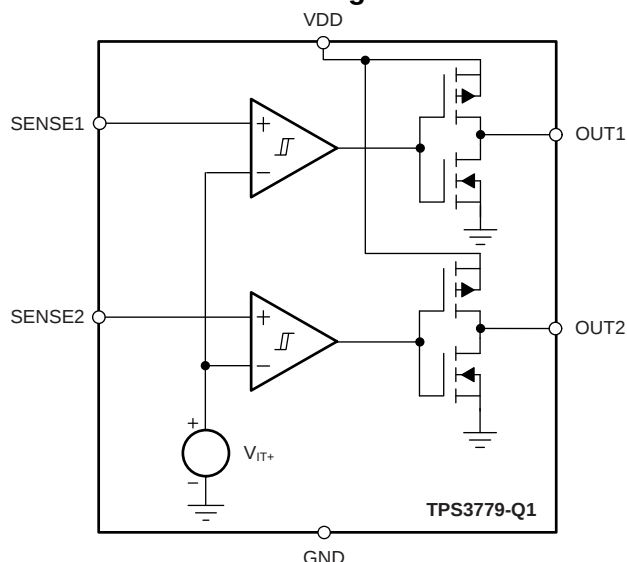
Figure 20. TPS3779-Q1 Block Diagram
