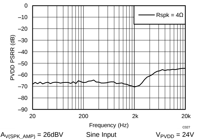
Figure 53. PVDD PSRR vs Frequency – PBTL
