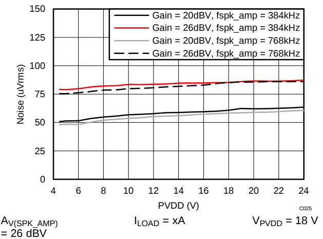
Figure 51. Idle Channel Noise vs PVDD – PBTL
