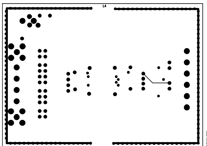
Figure 8. Internal Layer 4
