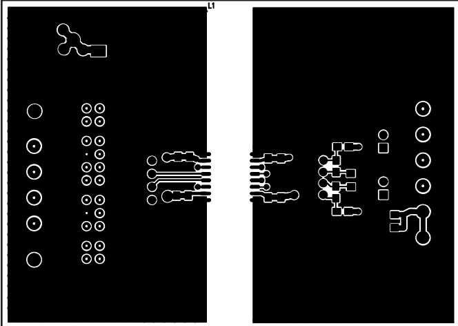
Figure 4. Top Layer
