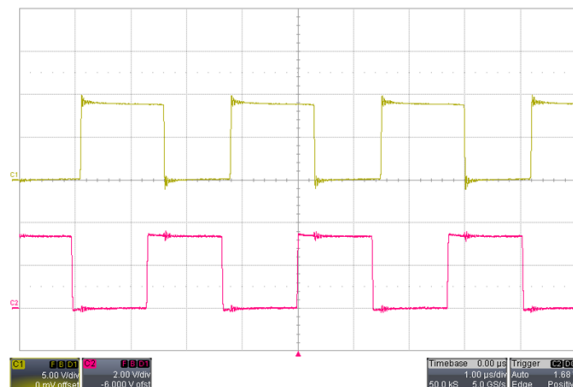
Figure 4. Clock Synchronization(C1:Switch node, C2:SYNC)
