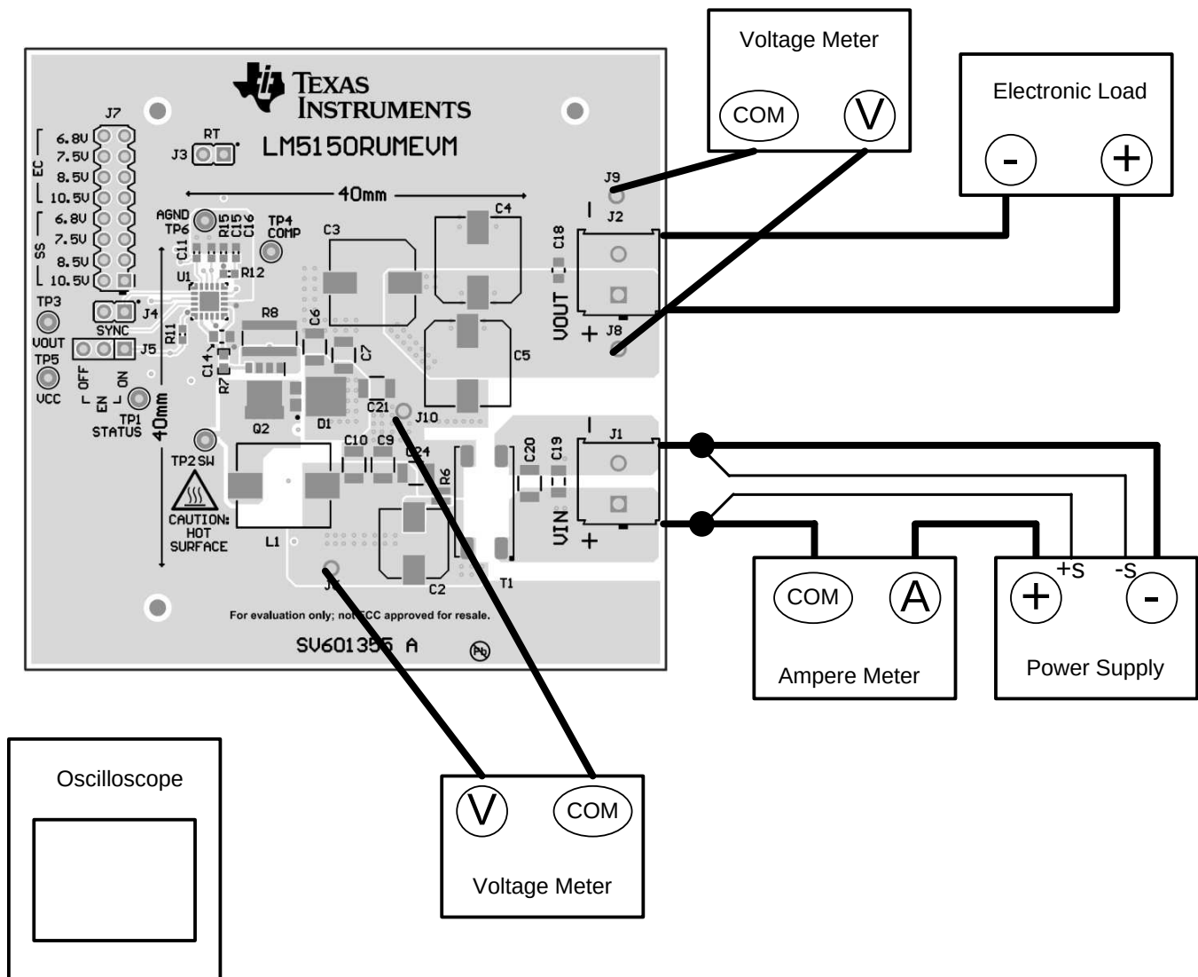
Figure 1. Standard Connection Diagram
