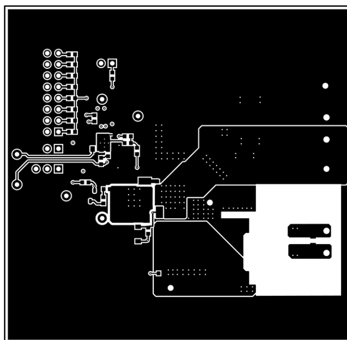
Figure 16. Bottom Copper (X-Ray View)
