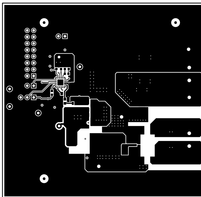
Figure 13. Top Copper (Top View)
