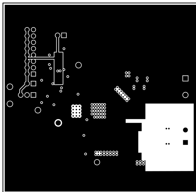
Figure 14. Mid1 Copper (X-Ray View)
