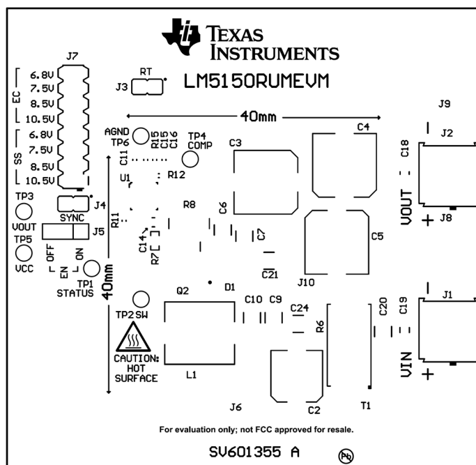
Figure 11. Top Silk (Top View)
