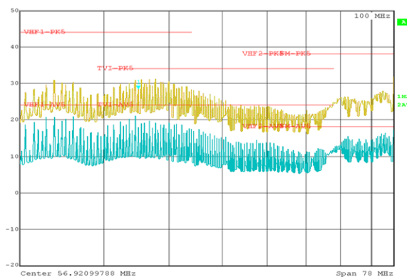
Figure 9. Conducted EMI Test Result 30MHz to 108MHz
