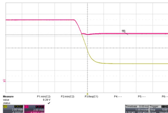
Figure 5. Cold-Cranking Using Cranking Simulator(C1: V_{SUPPLY} , C2: V_{LOAD} )
