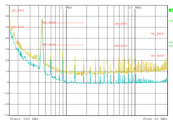
Figure 8. Conducted EMI Test Result 150kHz to 30MHz
