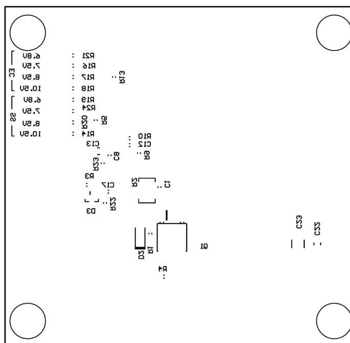
Figure 12. Bottom Silk (X-Ray View)
