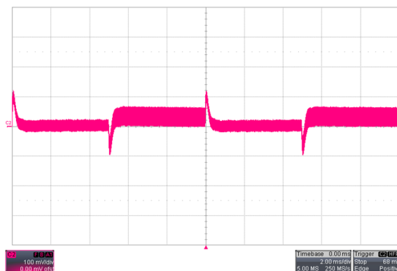
Figure 7. Load Transient(C2:V LOAD AC-coupled)
