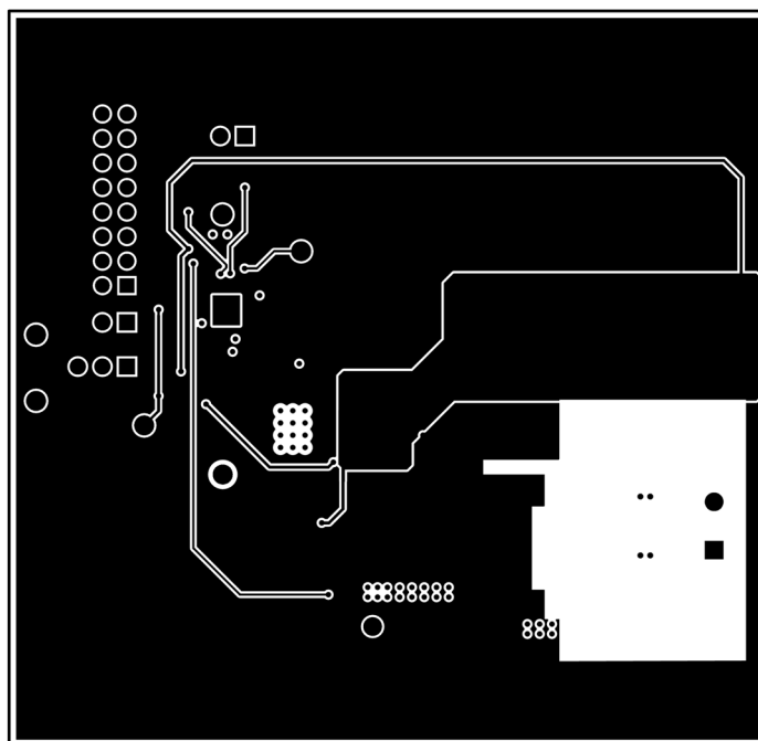
Figure 15. Mid2 Copper (X-Ray View)
