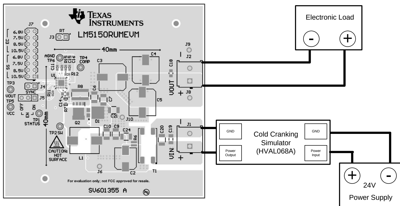
Figure 2. Cranking Simulator Connection Diagram
