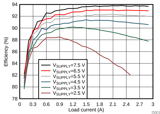
Figure 3. Efficiency
