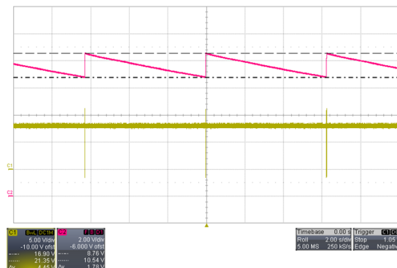
Figure 6. No Load Skip Cycle Operation(C1:Switch Node, C2: V_{LOAD} )
