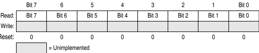
Figure 15-6. TIM Counter Low Register (TCNTL)
