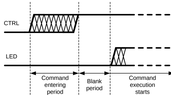
Figure 8. Single-Wire Interface
