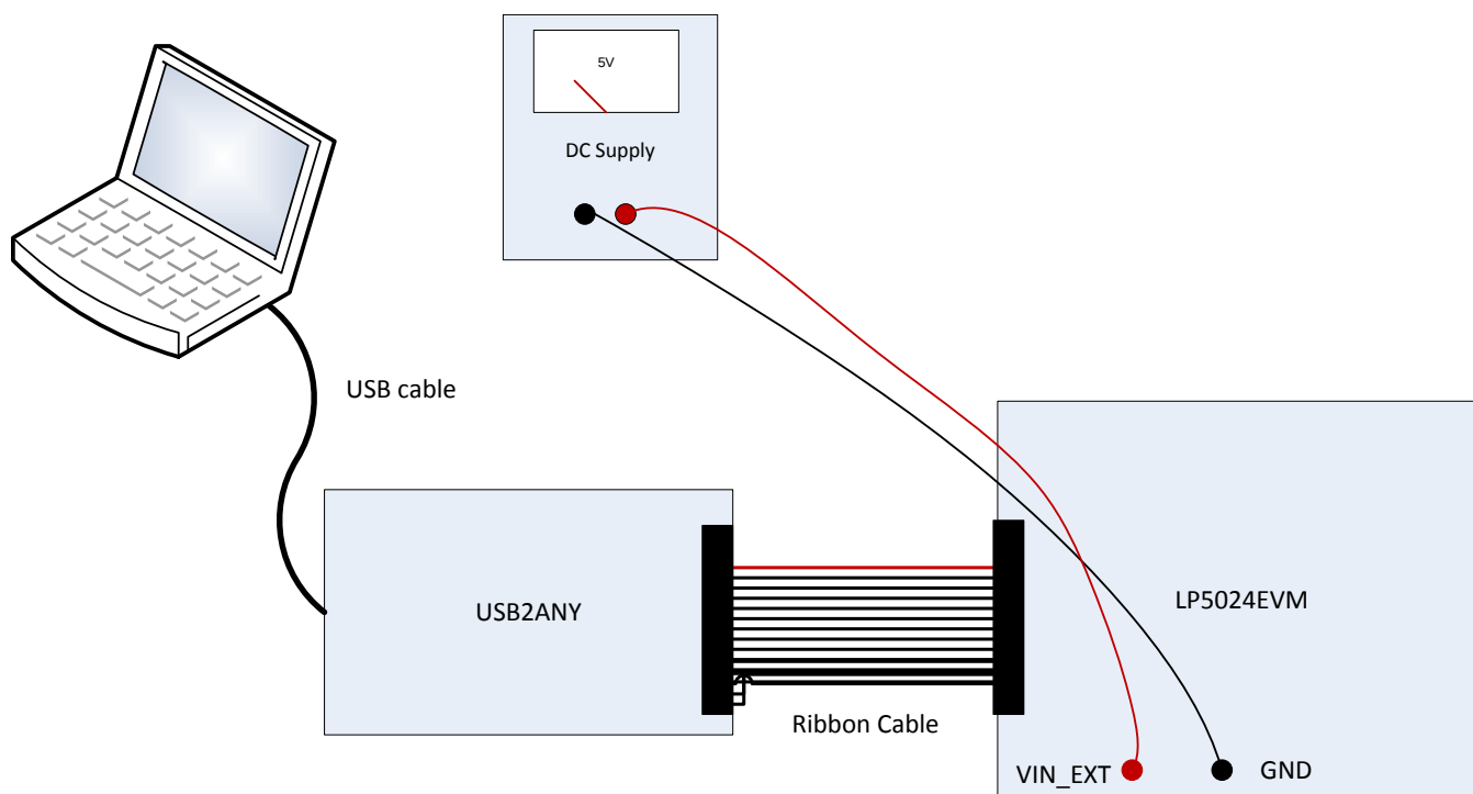
Figure 3. LP5024EVM Hardware Setup
