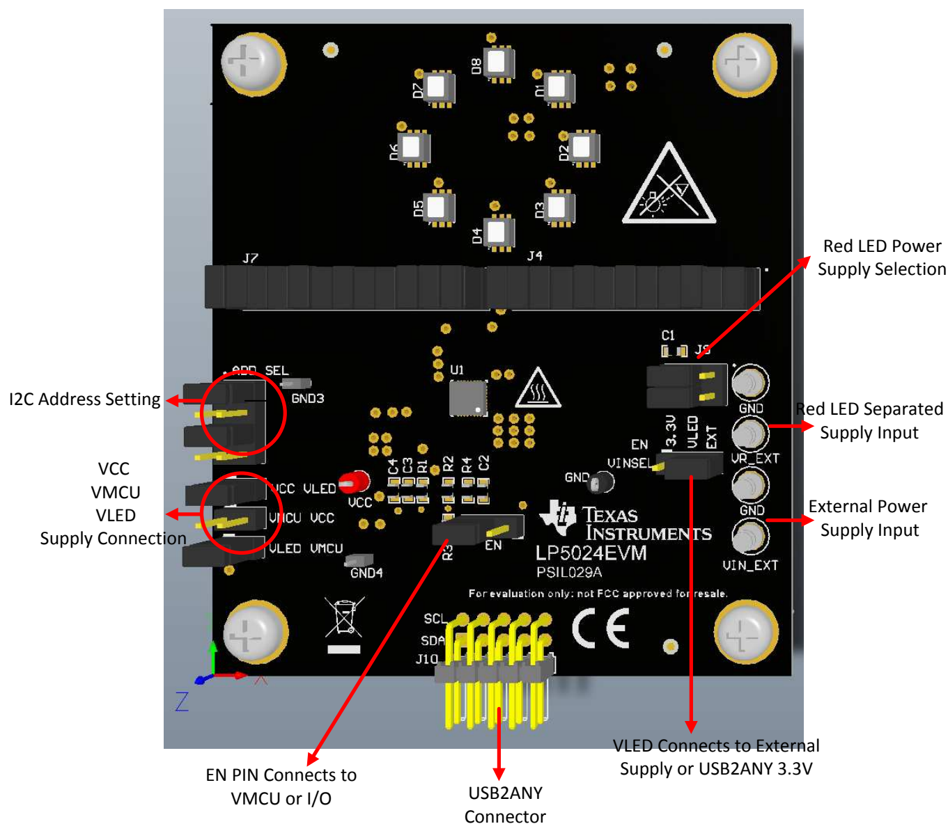
Figure 2. LP5024EVM Key Connectors
