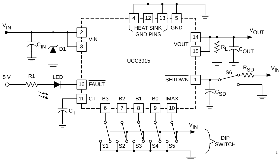
Figure 1. Evaluation Circuit
