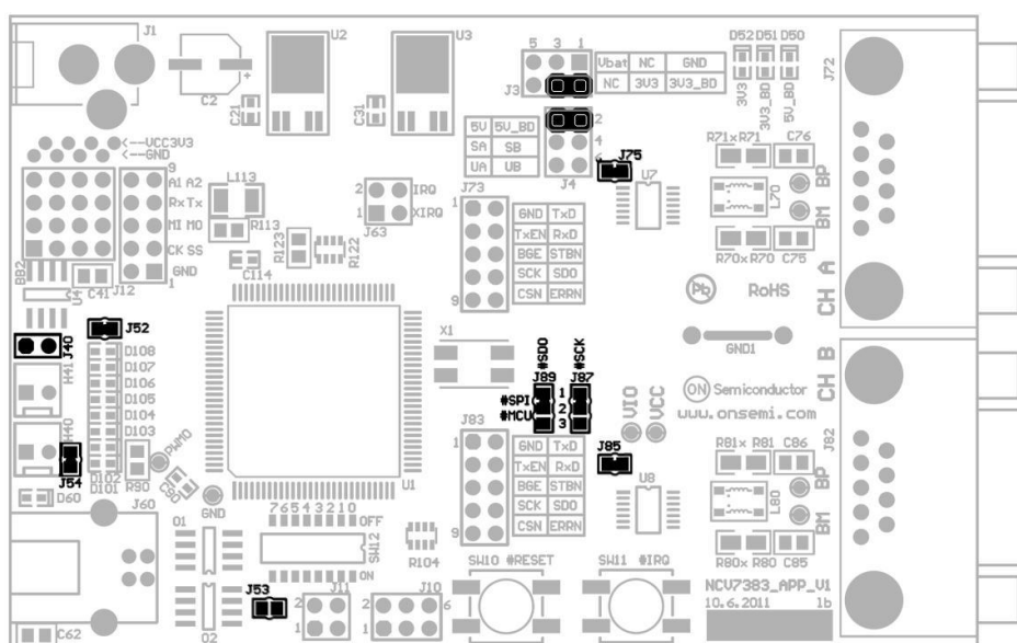
Figure 5. Jumpers and Soldering Straps
