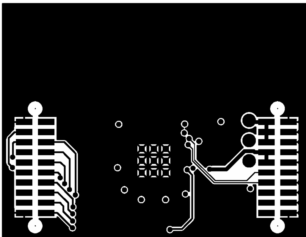
Figure 5: CC2420EM PCB layout, layer 4
