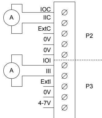
Figure 8: Power terminal block with amperemeters attached
