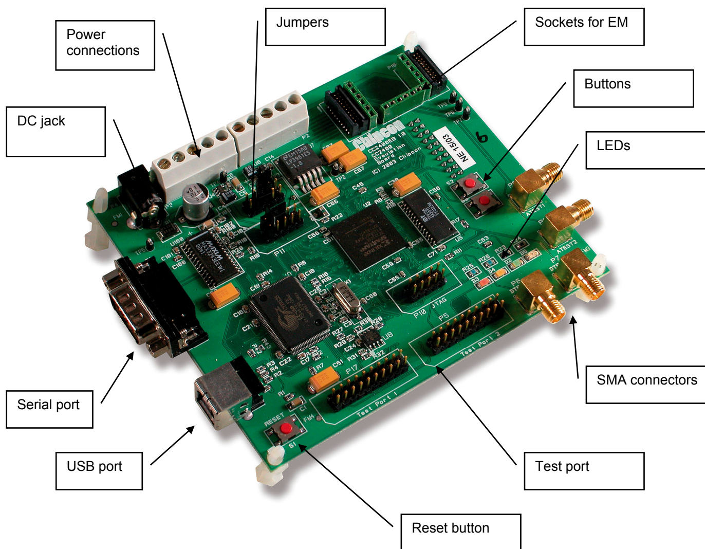
Figure 7: CC2400EB Evaluation Board
